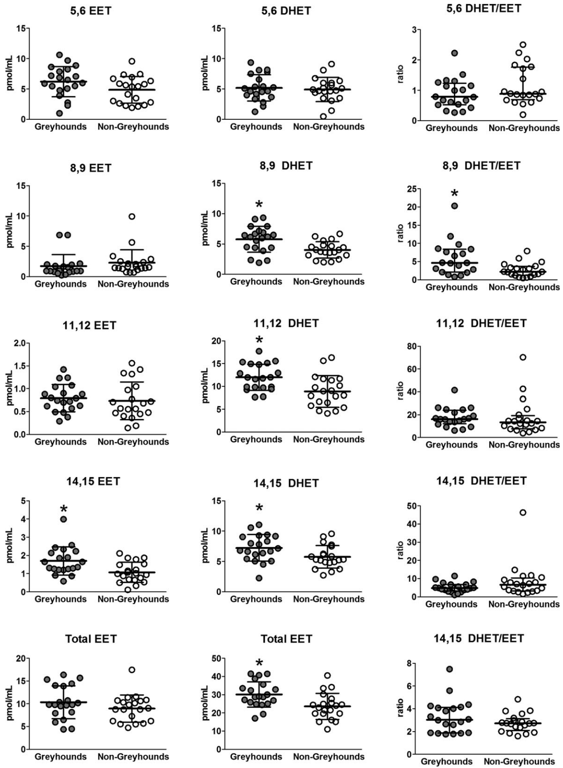
Fig 4. CYP450 epoxygenase metabolites of arachidonic acid (epoxyeicosatrienoic acids, EET) and their soluble expoxide hydrolase metabolites (dihydroxyeicosatrienoic acids, DHETs) in Greyhounds and non-Greyhound dogs. Filled circles are Greyhounds. Open circles are non-Greyhounds. The horizontal bars represent the mean \pm SD for the EETs and DHETs. Horizontal bars represent the median and interquartile range for the ratios. Significant difference indicated with ( *P < .033 ).
